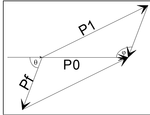
Vector description of the Cherenkov radiation.
